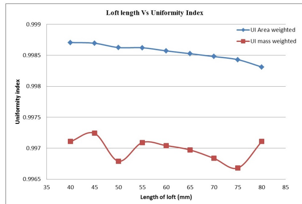
Fig. 10: Variation in uniformity index with loft length.
